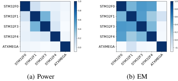
Figure 2: Evaluation of device variations for ST and AVR microprocessors using different side-channel sources.
