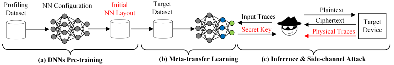
Figure 1: Overview of the proposed meta-transfer framework for profiled side-channel attacks: (a) Pre-training the DL model on the labelled profiling dataset; (b) Fine-tuning the trained DL model on target dataset using the meta-transfer learning; (c) Applying DL models on newly collected side channel traces from the target devices.
