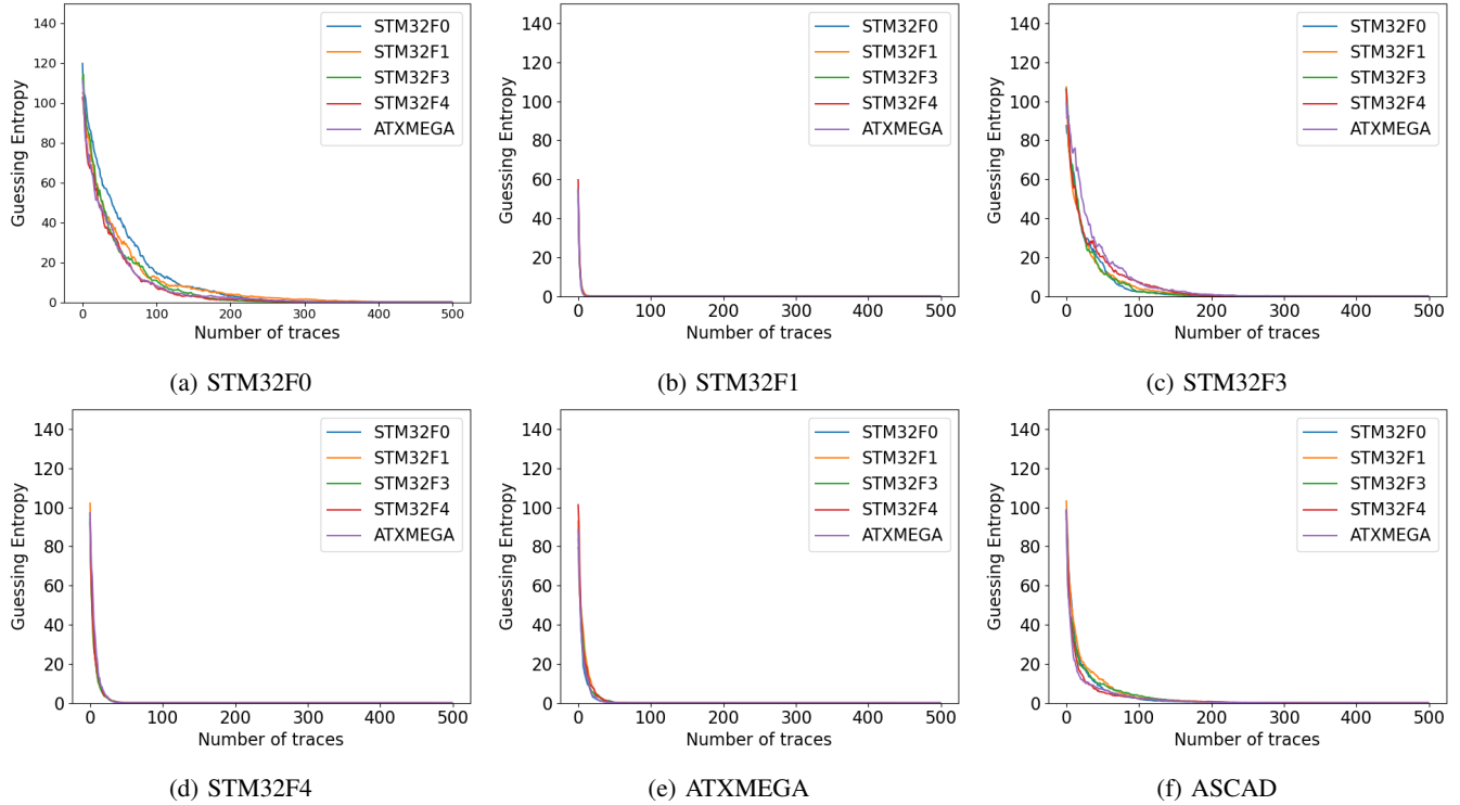
Figure 4: Experimental results of MTL-SCA on cross-device cross-domain attacks among different devices.
