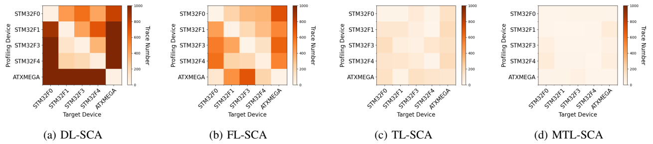
Figure 3: Comparisons of different cross-device side channel attacks.
